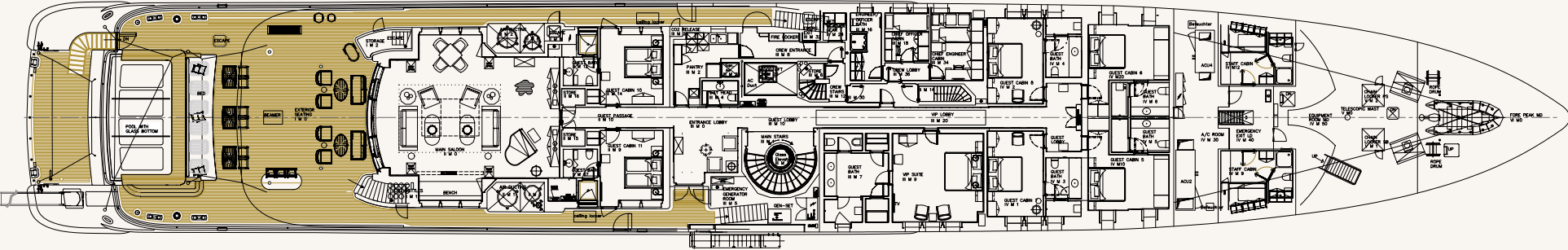
MAIN DECK
